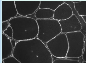
\beta SG
