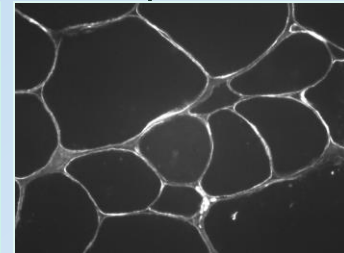
\beta DG
