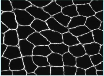
\alpha SG
