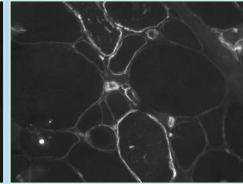
Utrophin
