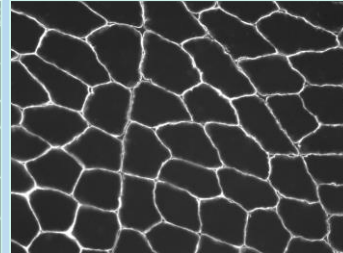
\gamma SG
